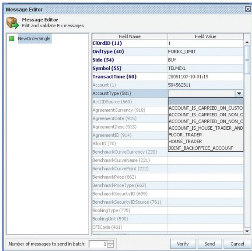
Sample Screens of the OMS Simulator Module
